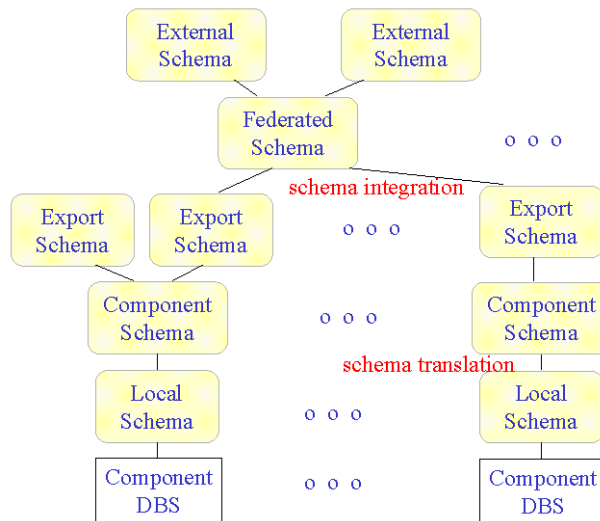
Figure 2. Schema architecture for a federated database system
