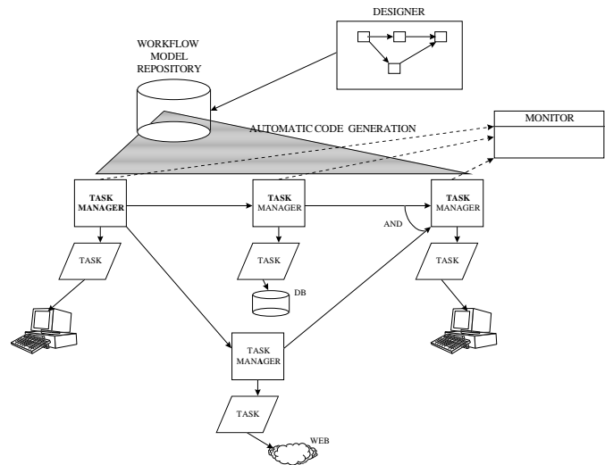
Figure 1: The METEOR Model
